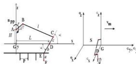
Figure 1. a - Kinematics of a point from the complex aggregate blade-bearing bar, the running mechanism; b - mobile and stationary reference
